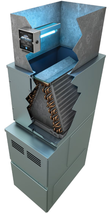
APCO ® RT Installed in Furnace
